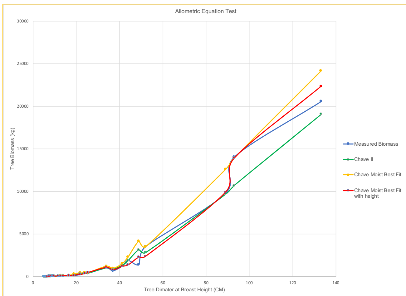
Figure 10: Destructive biomass measurements from the Cheko study and the Keo-Seima REDD+ Project compared to the predicted biomass values from 3 models from Chave et al. (2005) that were evaluated for best fit. The Chave model II.2 was shown to be the best fit and was selected for validation and use in the SCRP.
