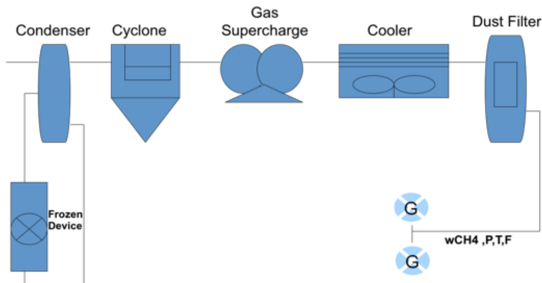
Figure B.2, the simplified diagram of pre-processing treatment layout.
