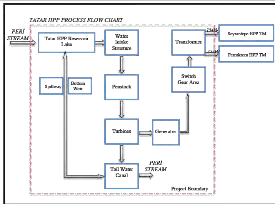
Figure 1: Basic Operational Principles of the Project Activity
