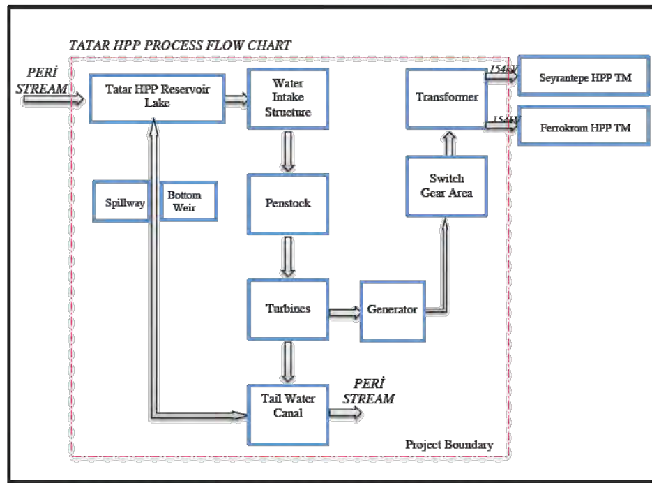
Figure 1: Basic Operational Principles of the Project Activity
