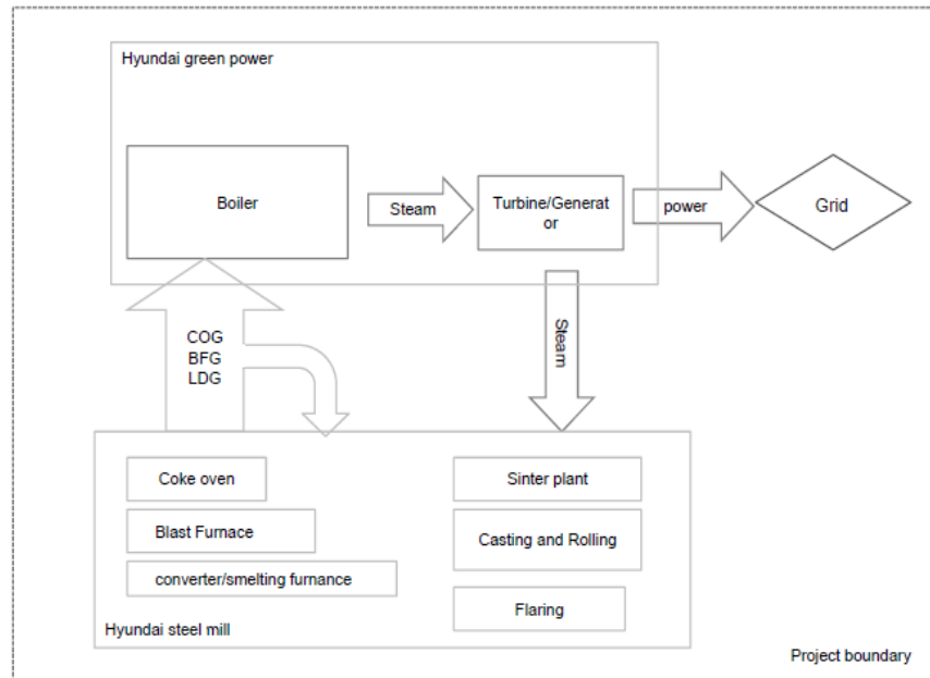
Figure 5. Baseline and project scenario diagrams
