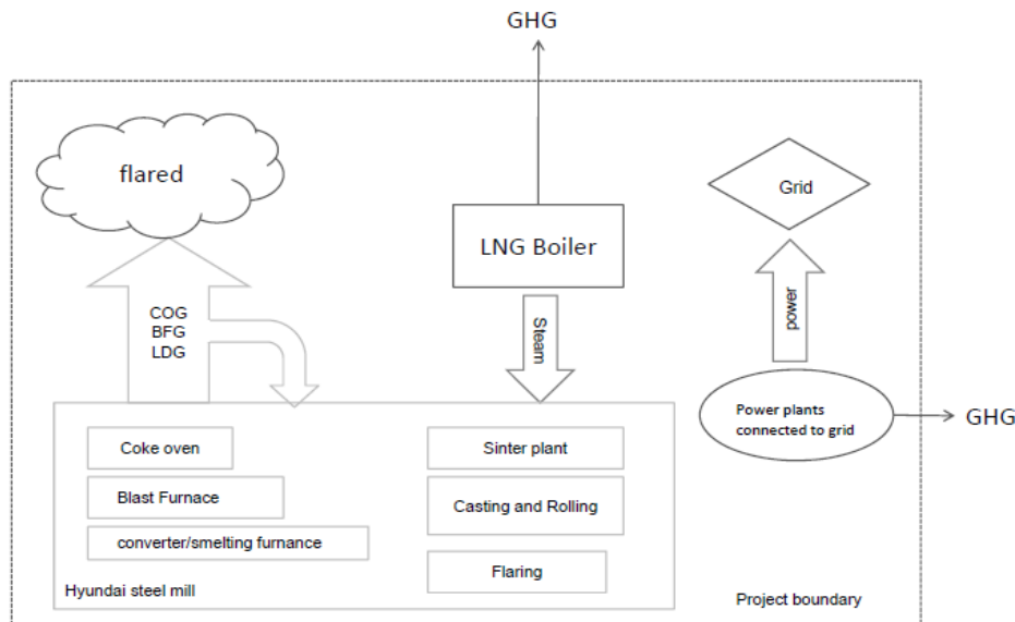
Process flow diagram baseline scenario
