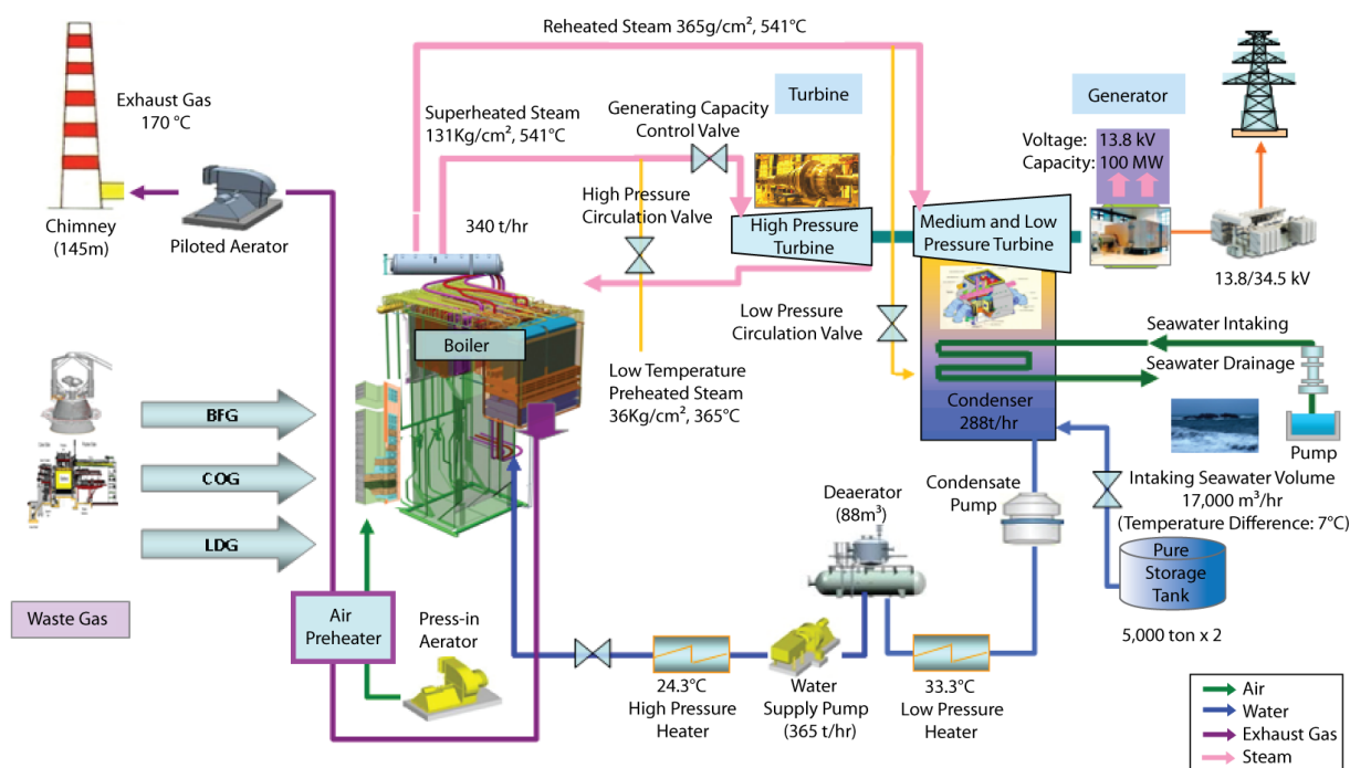
Figure 1. Project Activity Flow Chart
