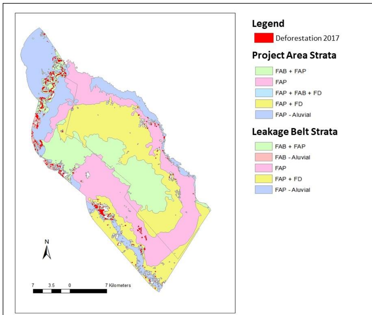
Figure 1.21. Map of 2017 deforestation in the project area and leakage belt.
