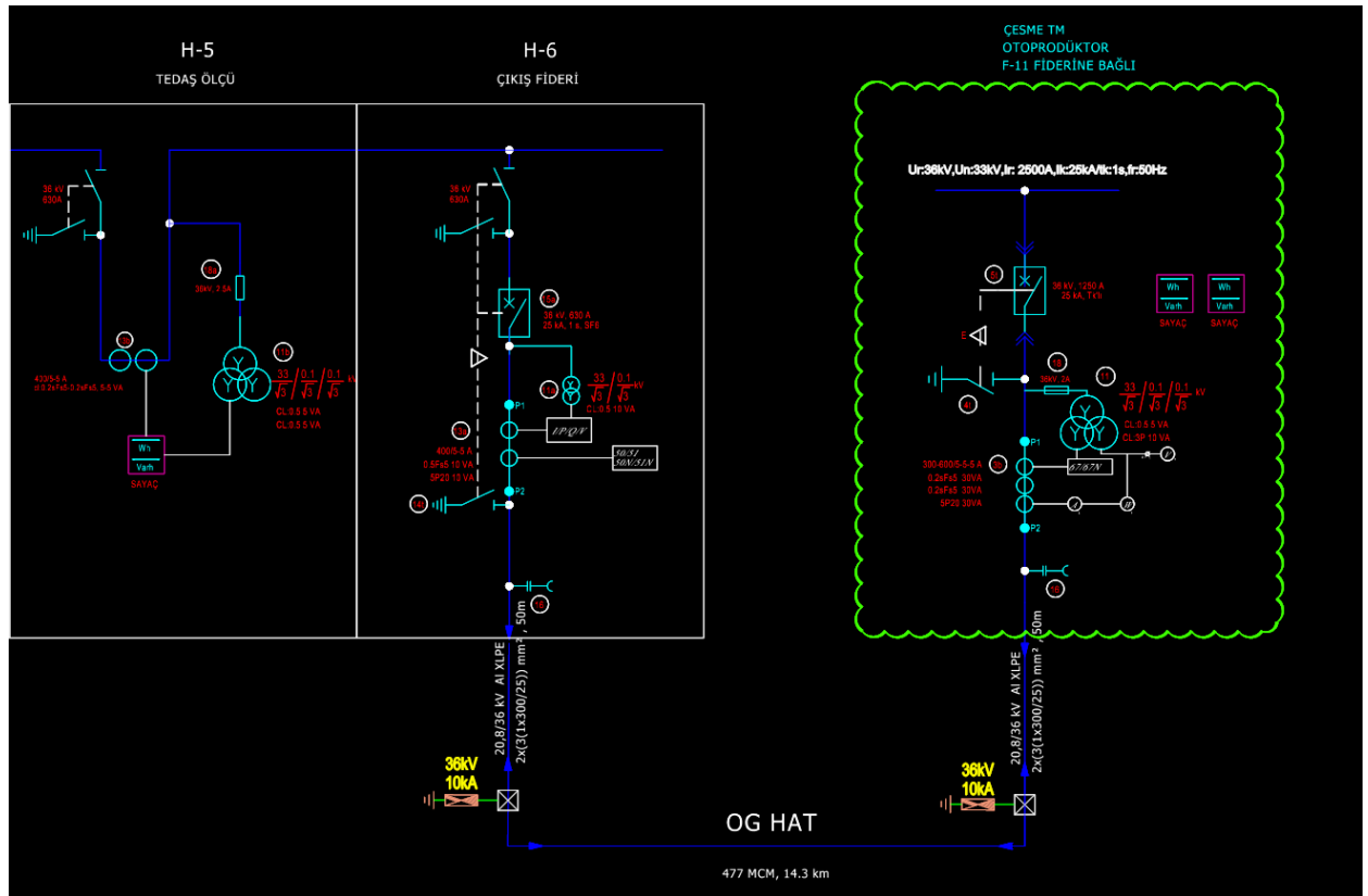
Figure 1: Single line diagram of Urla WPP
