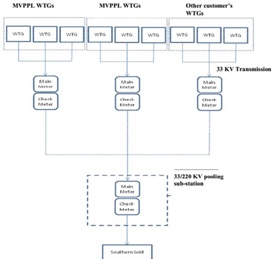
Figure 2. Schematic diagram indicating the metering system
