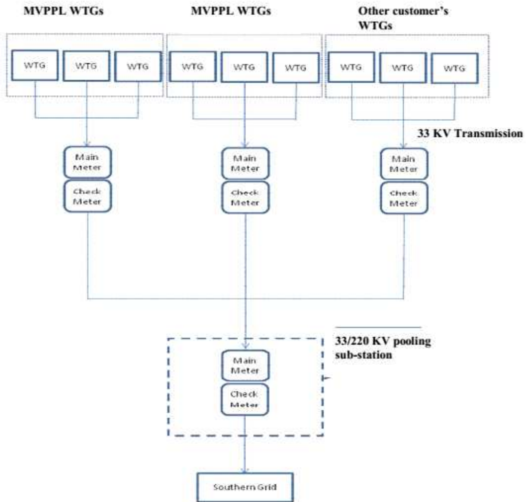
Figure 2. Schematic diagram indicating the metering system
