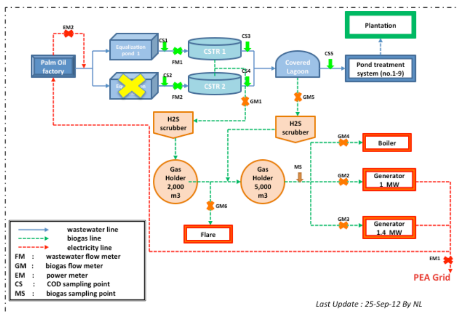
Figure 3 : Monitoring diagram
